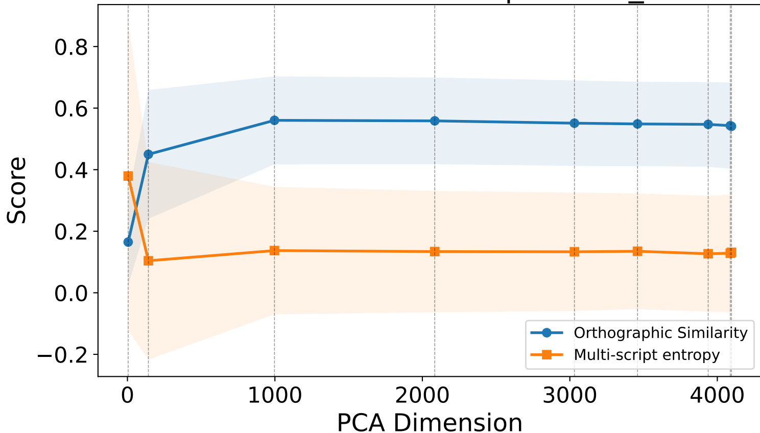
mistralai/Mistral-7B-v0.1 | mcs=5_ms=6
